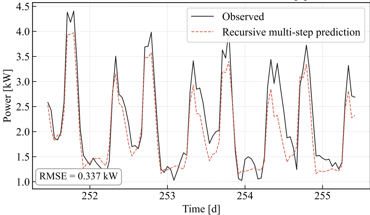
Validation set — observed vs. recursive multi-step prediction
